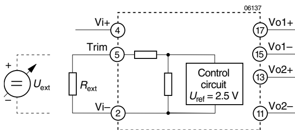
Fig. 15 Output voltage control for Quad (double) output units by means of the Trim input on the primary side.
