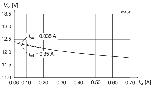
Fig. 9 Cross load regulation V_{o4} versus I_{o1} (typ) for various I_{o4} for Vo1 , Vo4 on power train 1. See: Block diagram dual output types. (20IMX35D12D12-9)
