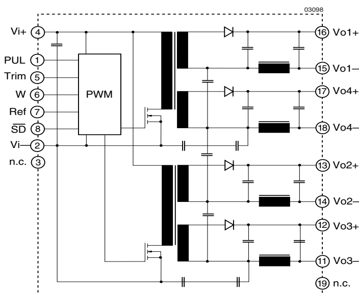
Fig. 2 Block diagram, quadruple output types
