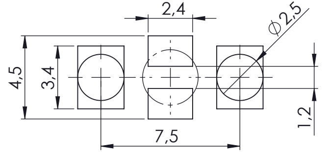
Layout Suggestion
