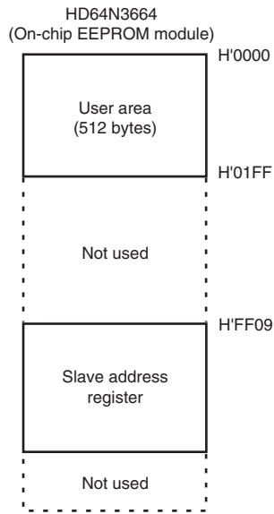
Figure 2.1 Memory Map (3)
