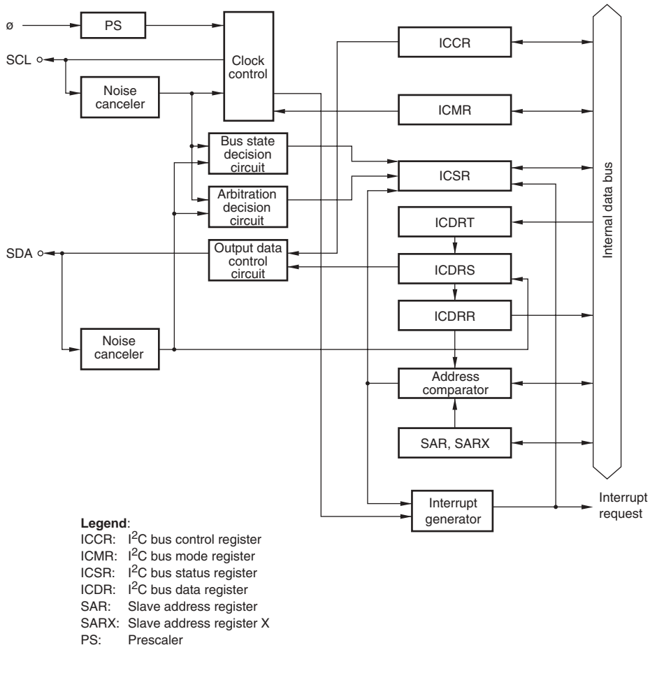
Figure 15.1 Block Diagram of I 2 C Bus Interface
