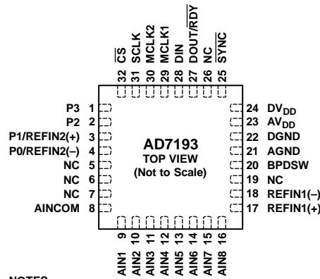
Figure 6. 32-Lead LFCSP Pin Configuration
