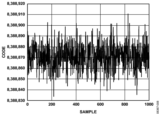
Figure 9. Noise ( V_{REF} = AV_{DD} = 5\text{ V} , Output Data Rate = 2400 Hz, Gain = 1, Chop Disabled, \text{Sinc}^4 Filter)
