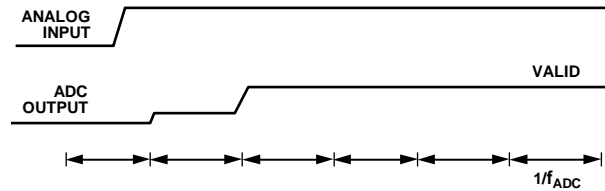
Figure 56. Step Change on Analog Input, Sinc 4 Filter
